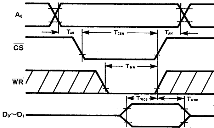
Fig. A-1 Write Timing
